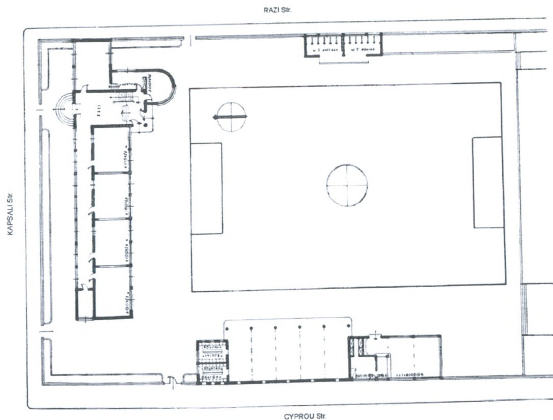
Fig.1 Ground floor plan (original drawing).
