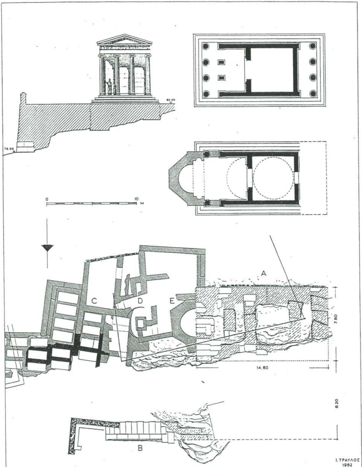
156 Temple of Artemis Agrotera, 448 B.C., restored elevation and plan. Plan of the temple as Christian church A. Foundations of the temple - B. Retaining wall - C. Christian graves - D. Apse of the early Christian church - E. Apse of the 17th c. church.
