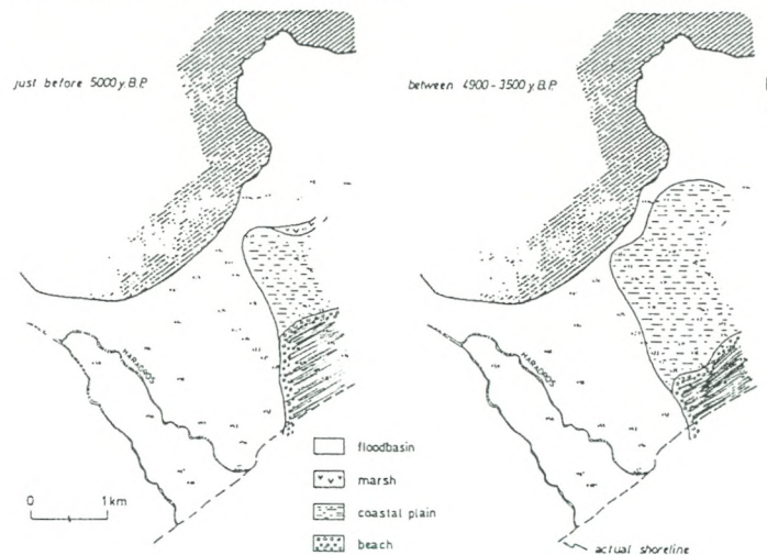
Figure 11. Paleogeographical reconstruction of the Shinias area in the periods just before 5000 BP and between 4900 to 3500 BP showing the situation of the shorelines and the extension of the coastal plain.
